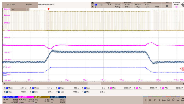
V_{IN} = 5.0V TPS6286A10 V_{OUT} = 0.9V BOM = 4 \times 22 \mu F I_{OUT} = 4A 至 10A
