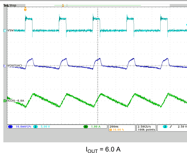
图 9-12. PWM Operation
