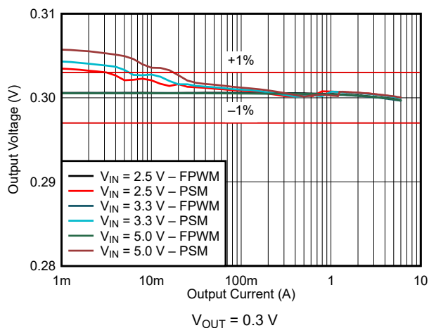
图 9-22. Load Regulation
