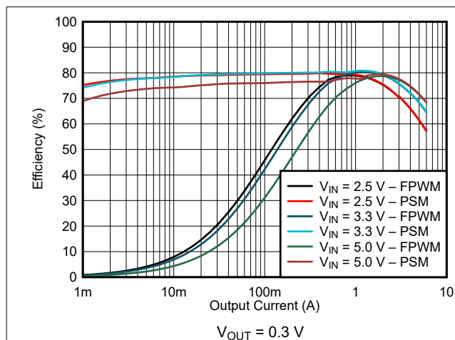
图 9-21. Efficiency
