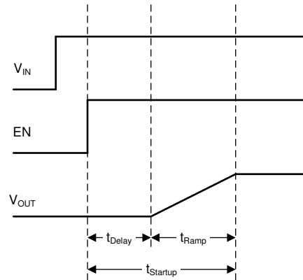
图 7-1. Start-up Sequence
