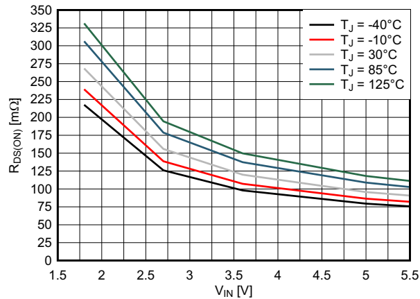
图 6-3. High-side Switch Drain Source Resistance R_{DS(ON)}
