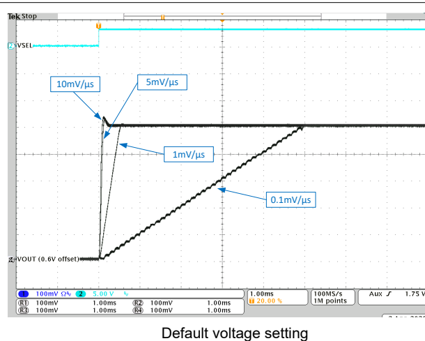
图 9-12. DVS by VSEL, Different Ramp Speed Settings
