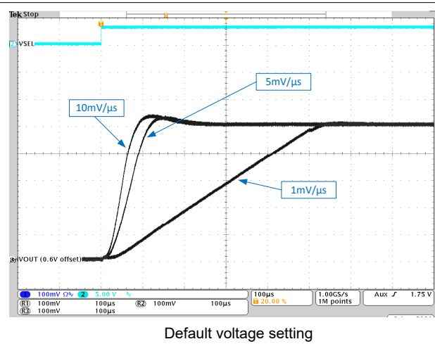
图 9-13. DVS by VSEL, Different Ramp Speed Settings
