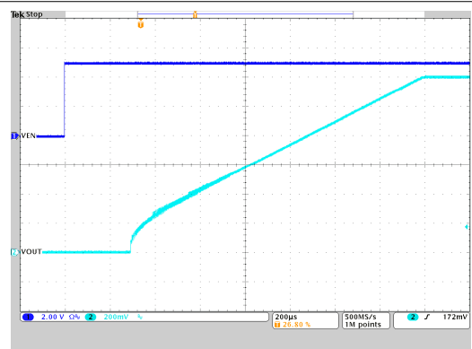
图 10-52. Start-Up Timing
