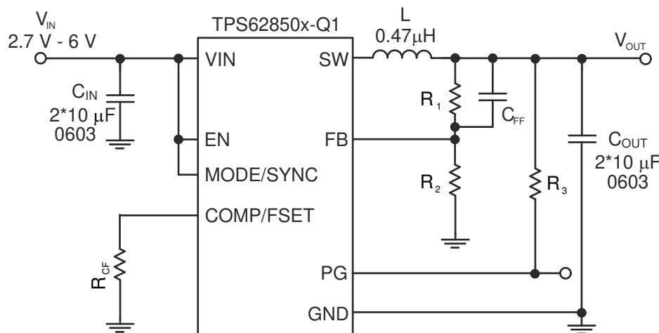
图 9-1. Typical Application
