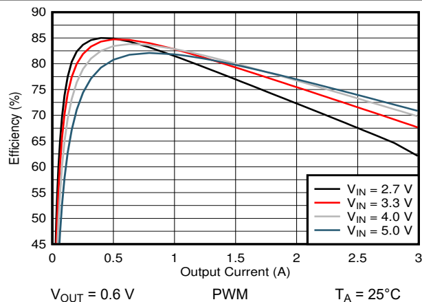
图 9-9. Efficiency Versus Output Current
