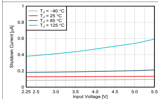
图 6-3. Shutdown Current
