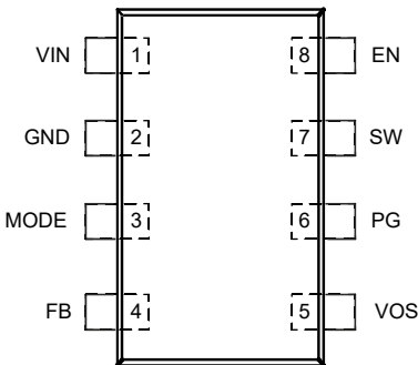
图 5-2. DRL Package 8-Pin SOT Top View
