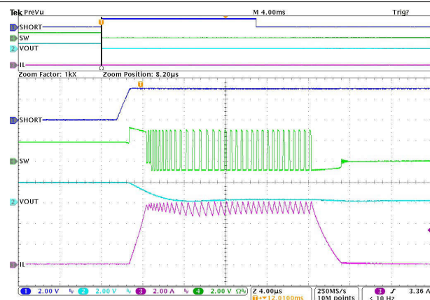
图 8-45. HICCUP Short-Circuit Protection (Zoom In - Second Hiccup)
