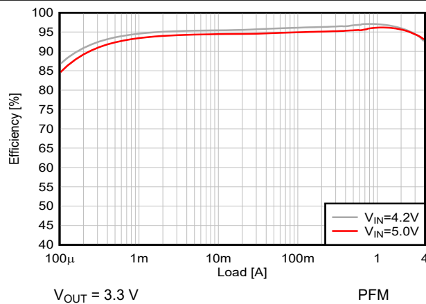
图 8-3. Efficiency versus Output Current
