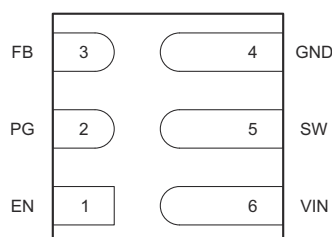
图 5-1. DMQ Package, 6-Pin VSON-HR (Bottom View)
