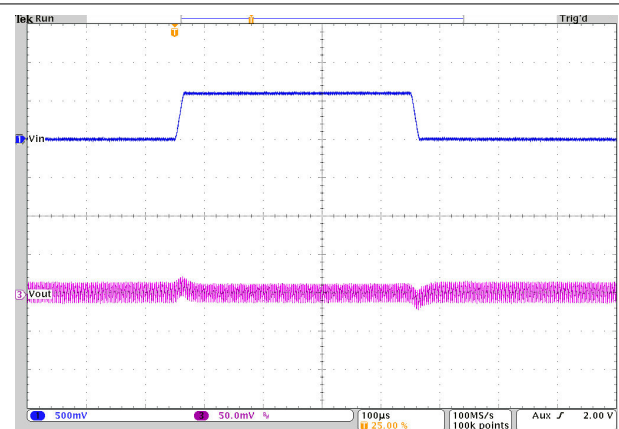
图 10-38. Line Transient Response
