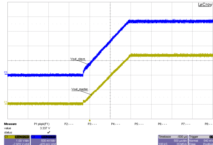
图 10-58. Scope Plot for Output Voltage Tracking
