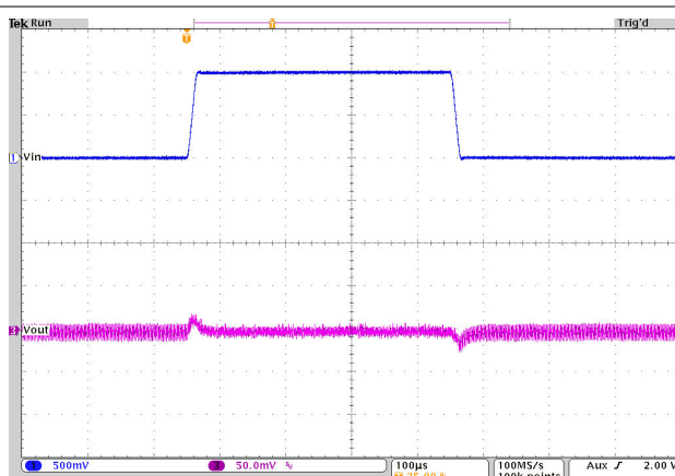
图 10-34. Line Transient Response
