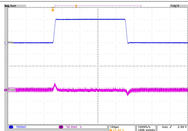
图 10-32. Line Transient Response
