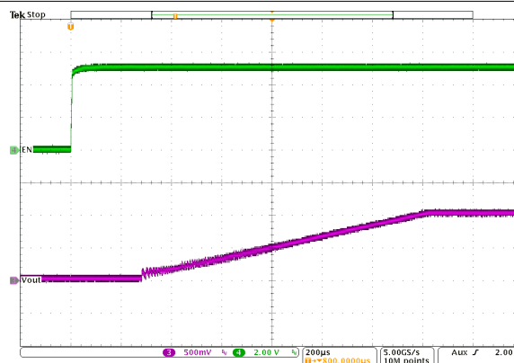
图 10-53. Start-Up Timing
