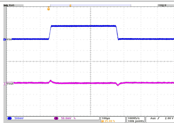
图 10-39. Line Transient Response
