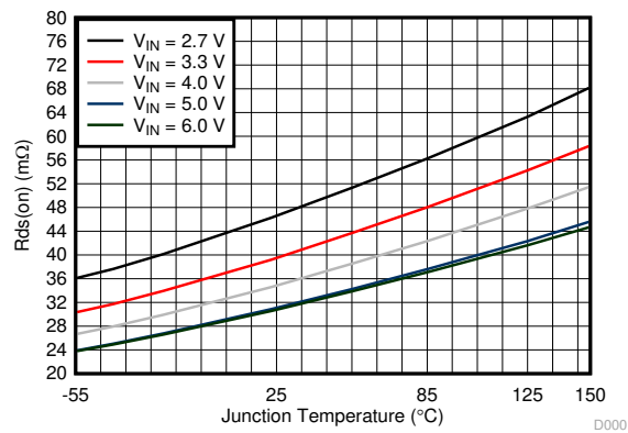
图 7-1. R_{ds(on)} of High-side Switch
