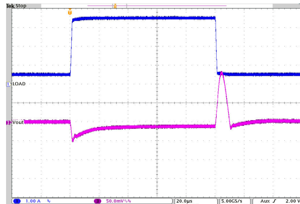
图 10-29. Load Transient Response
