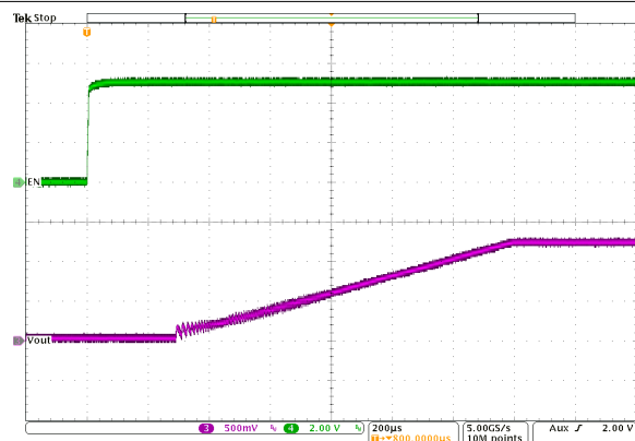
图 10-52. Start-Up Timing
