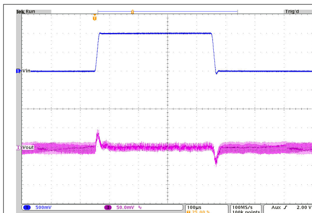
V_{OUT} = 3.3V PFM T_A = 25^{\circ}C I_{OUT} = 0.5A V_{IN} = 4.5V 至 5.5V 至 4.5V
