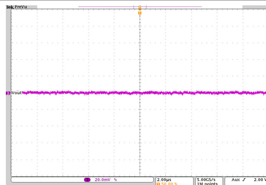
V_{OUT} = 0.6V PWM T_A = 25^\circ C I_{OUT} = 4A V_{IN} = 3.3V BW = 20MHz
