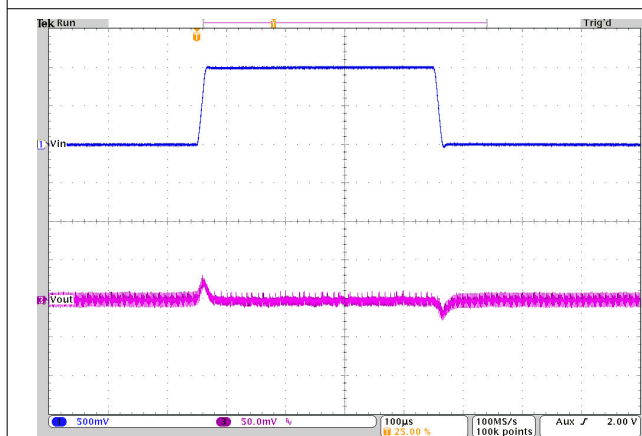
V_{OUT} = 1.8V PFM T_A = 25^{\circ}C I_{OUT} = 0.5A V_{IN} = 4.5V 至 5.5V 至 4.5V
