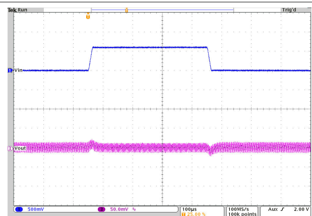
V_{OUT} = 0.6V PFM T_A = 25^\circ C I_{OUT} = 0.5A V_{IN} = 3.0V 至 3.6V 至 3.0V
