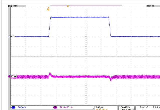
V_{OUT} = 1.2V PFM T_A = 25^{\circ}C I_{OUT} = 0.5A V_{IN} = 4.5V 至 5.5V 至 4.5V
