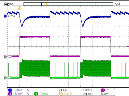
图 38. Transient Response VOUT2 = 5 V
