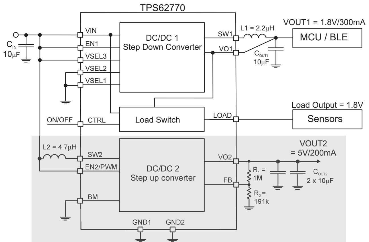
图 36. Step-Up Converter Providing 5-V VOUT2
