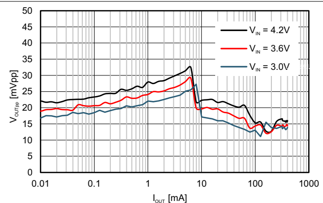
图 9-13. Typical Output Ripple Voltage V_{OUT} = 1.4\text{ V} L = 2.2\mu\text{H} C_{OUT} = 10\mu\text{F} (0402)
