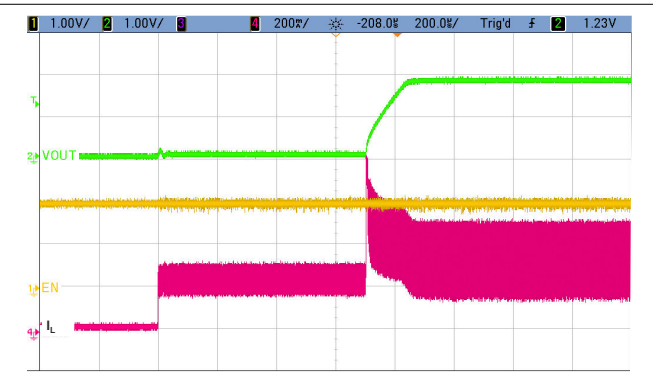
图 9-17. Startup Into 300 mA Electronic Load Soft-Start Delay
