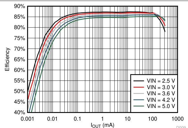
图 9-5. Efficiency vs Load Current; V_{OUT} = 1.8\text{ V}
