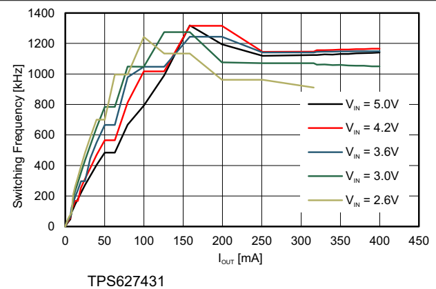
图 9-11. Switching Frequency vs Load Current V_{OUT} = 1.4\text{ V}
