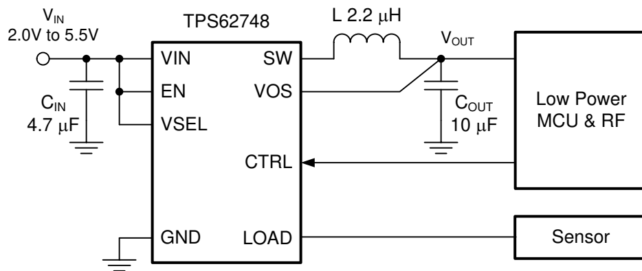
图 9-1. TPS62748 Typical Application Circuit
