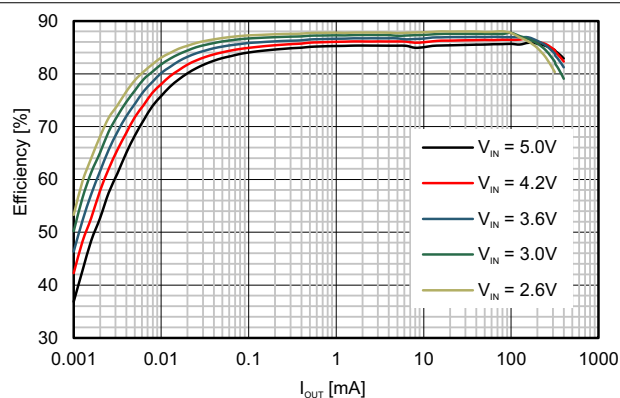
图 9-6. Efficiency vs Load Current; V_{OUT} = 1.4\text{ V}
