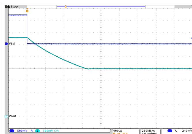
Figure 39. TPS62745 Output Voltage Change from 3.3 V to 2.0 V for I_{OUT} = 10 mA
