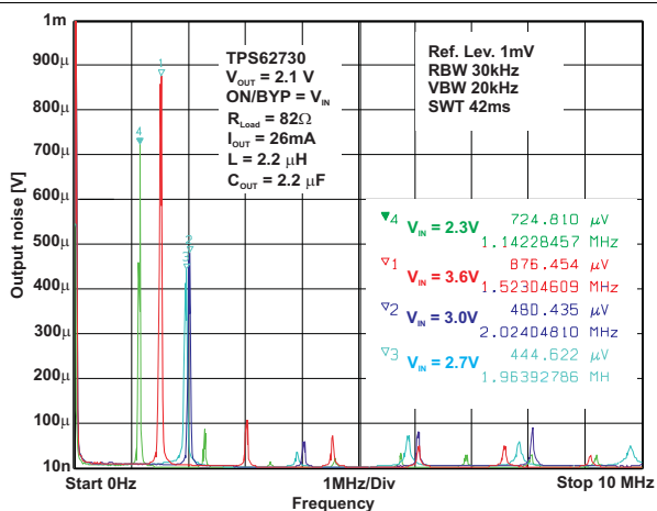
Figure 28. Spurious Output Noise TPS62730 I_{OUT} 26 mA
