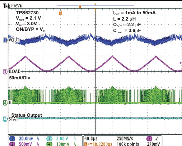
Figure 25. DC-DC Mode V_{OUT} AC Load Regulation Performance
