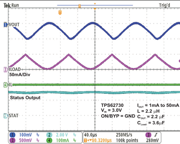
Figure 26. Bypass Mode Operation V_{OUT} AC Behavior ON/BYP = GND
