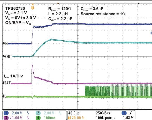
Figure 27. Start-Up Behavior
