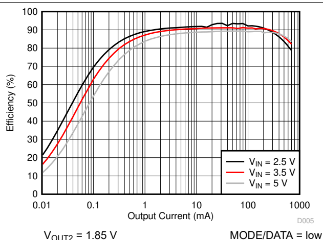
图 9-4. TPS62407-Q1 Efficiency, V_{OUT2}
