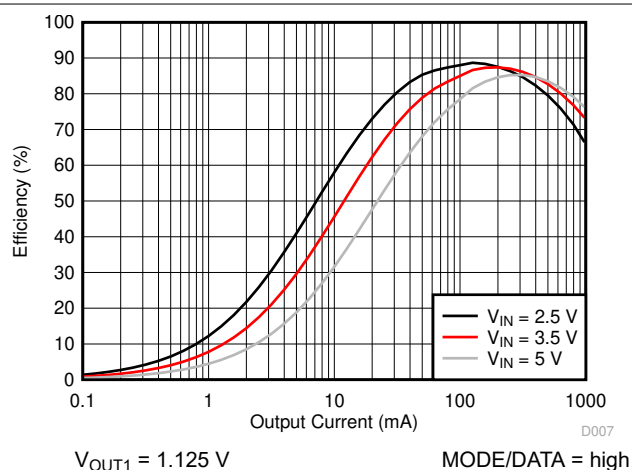
图 9-7. TPS62406-Q1 Efficiency, V_{OUT2}
