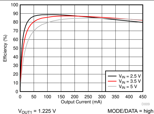
图 9-3. TPS62407-Q1 Efficiency, V_{OUT1}
