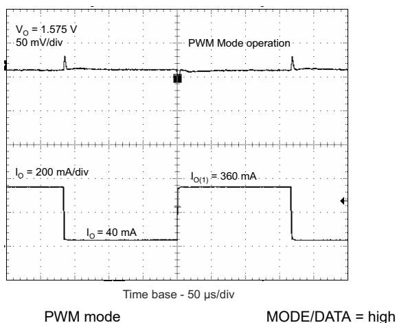
图 9-18. Load-Transient Response, PWM Operation
