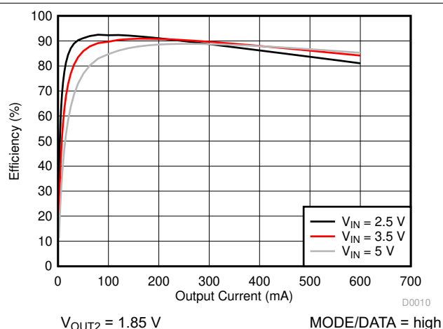
图 9-5. TPS62407-Q1 Efficiency, V_{OUT2}
