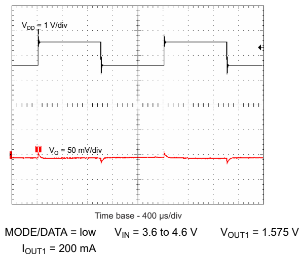
图 9-19. Line-Transient Response
