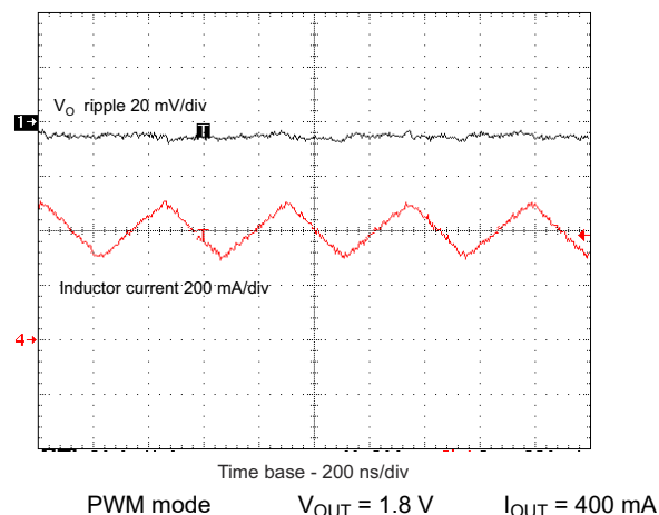
图 9-15. Output-Voltage Ripple in PWM Mode
