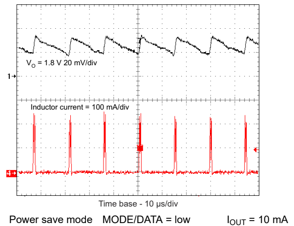
图 9-13. Light-Load Output-Voltage Ripple in Power-Save Mode
