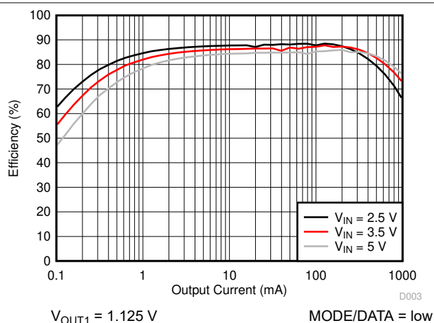
图 9-6. TPS62406-Q1 Efficiency, V_{OUT1}
