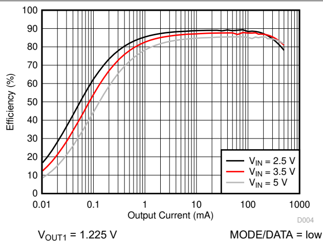
图 9-2. TPS62407-Q1 Efficiency, V_{OUT1}
