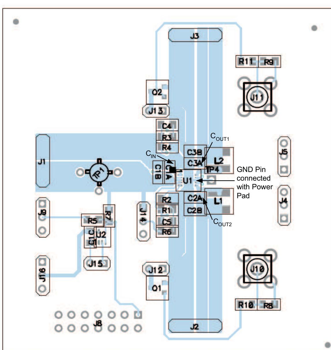
Figure 36. PCB Layout
