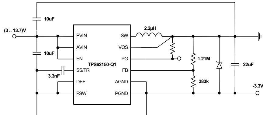
Figure 48. -3.3-V Inverting Power Supply
