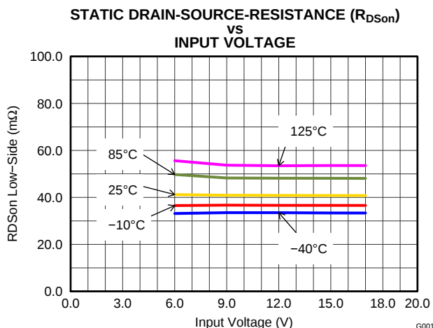
Figure 24. Low-Side Switch Resistance
