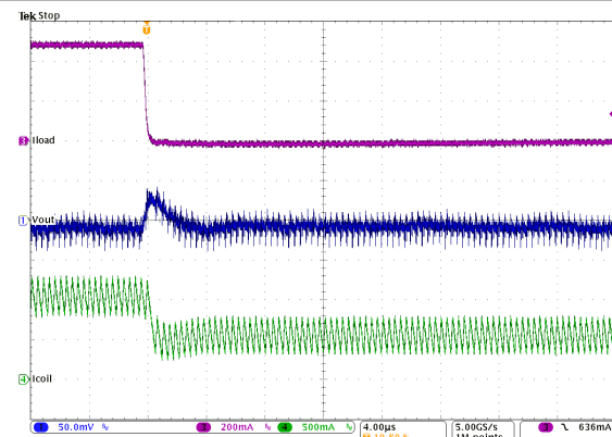
图 9-31. Load Transient Response
