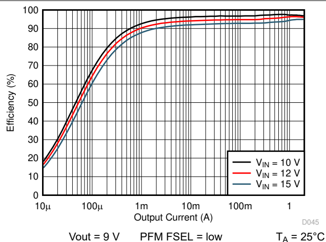
图 10-19. Efficiency vs Output Current
