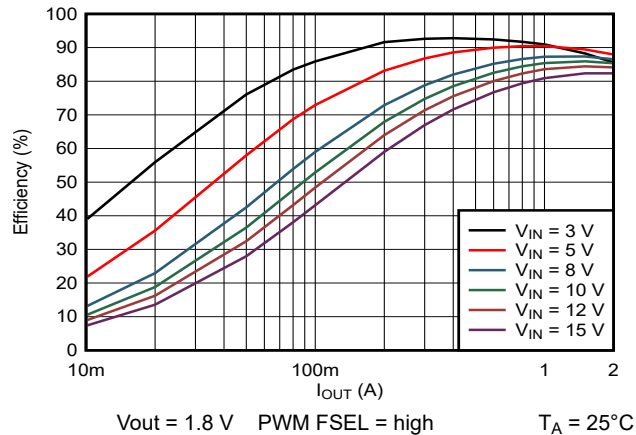
图 10-8. Efficiency vs Output Current
