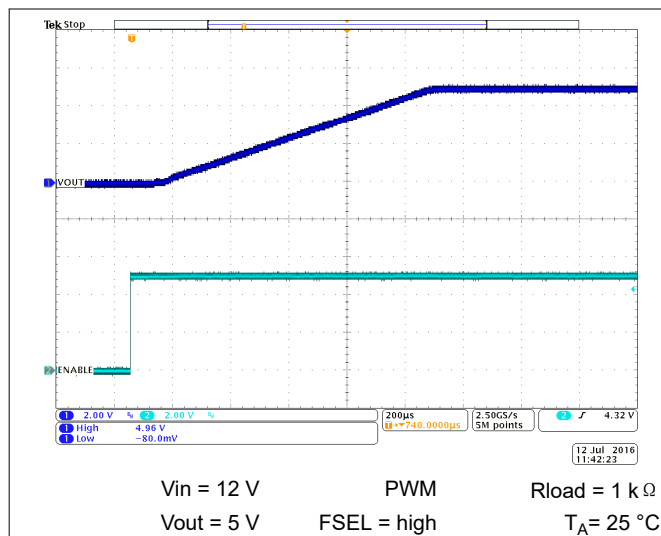
图 10-56. Start-Up Timing
