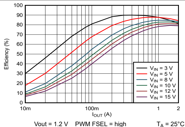
图 10-4. Efficiency vs Output Current
