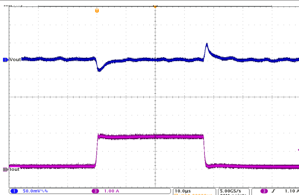
图 10-39. Load Transient Response
