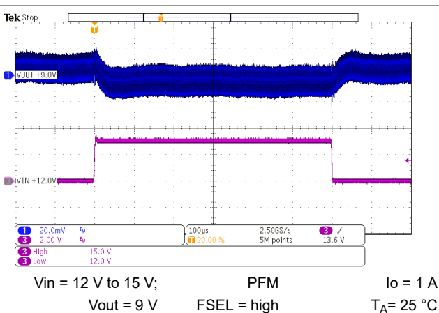
图 10-61. Line Transient Response
