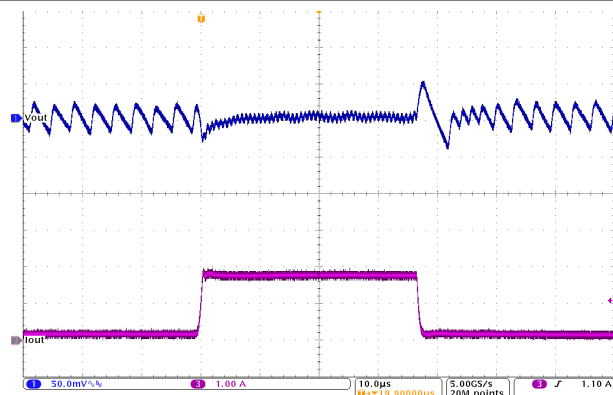
图 10-38. Load Transient Response
