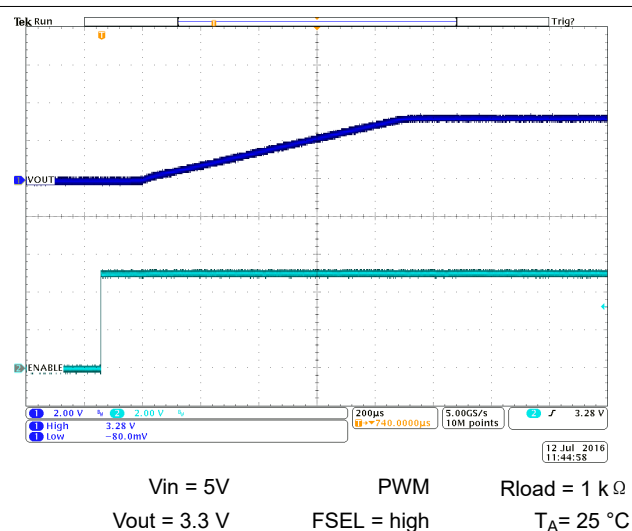
图 10-49. Start-Up Timing
