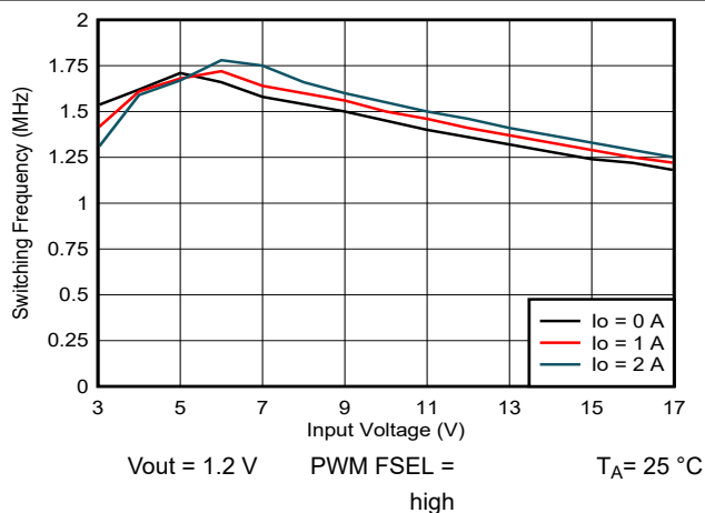
图 10-66. Switching Frequency vs Input Voltage
