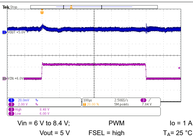
图 10-55. Line Transient Response
