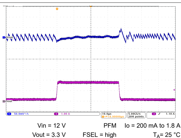
图 10-45. Load Transient Response
