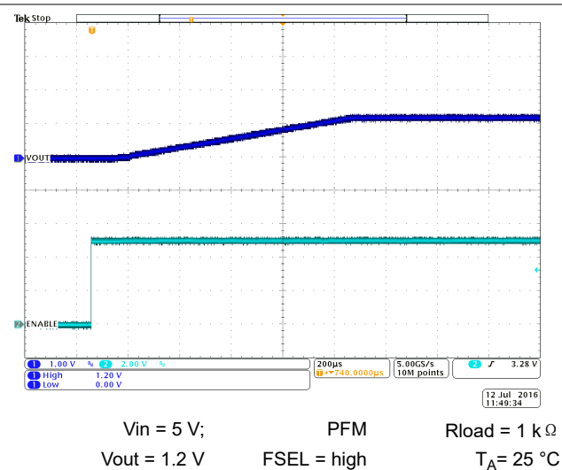
图 10-35. Start-Up Timing
