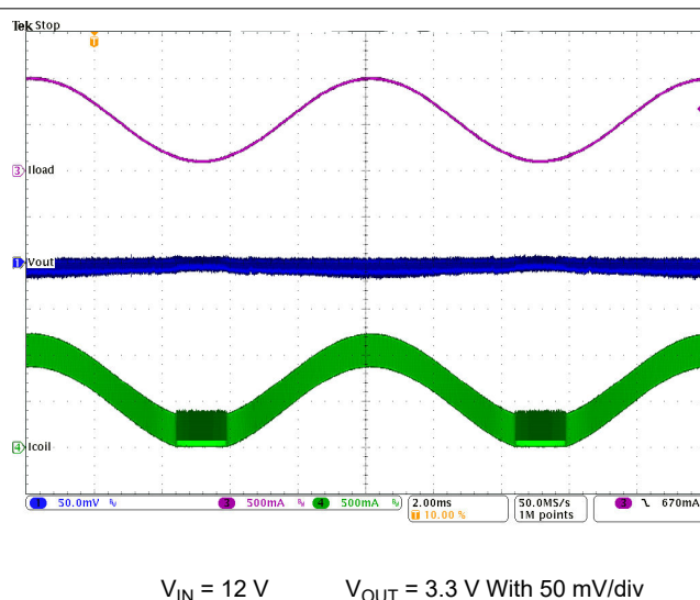
图 9-30. PWM-PSM-Transition
