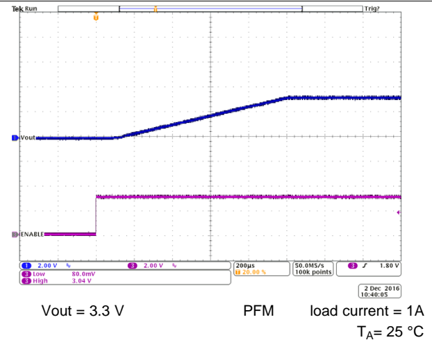
Figure 49. Start-Up Timing
