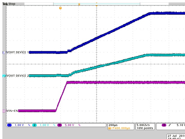
Figure 78. Tracking
