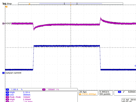
Vout = 5 V PWM I o = 350 mA to 3.1 A T A = 25 °C
