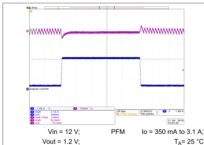
图 10-33. Load Transient Response
