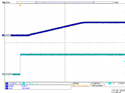
Vout = 3.3 V PWM Rload = 1 k \Omega T A = 25 °C
