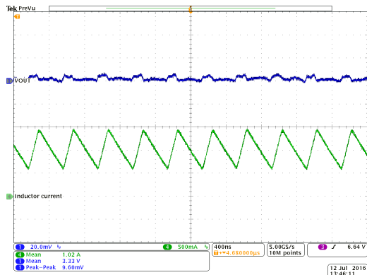
Vout = 3.3 V PWM I o = 1 A T A = 25 °C
