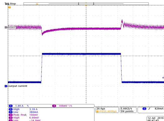
Vout = 5 V PFM I o = 350 mA to 3.1 A T A = 25 °C
