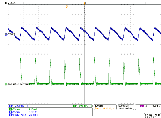
Vout = 3.3 V PFM I o = 0.1 A T A = 25 °C
