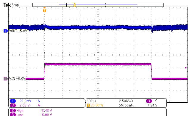
Vin = 6 V to 8.4 V; PFM I o = 1 A Vout = 5 V T A = 25 °C
