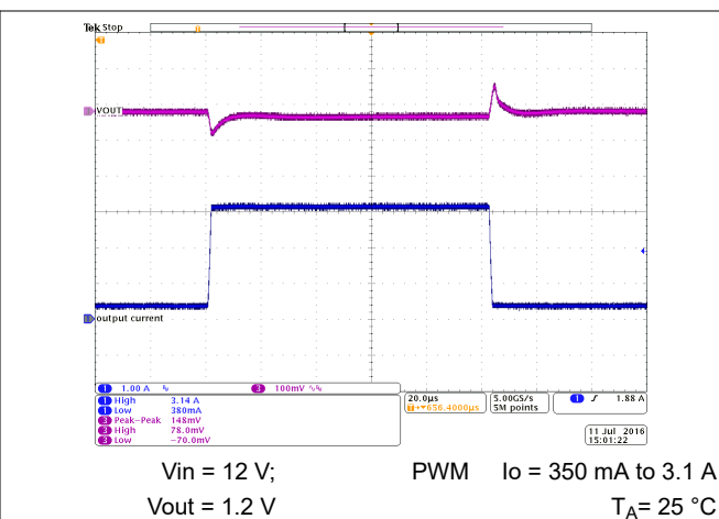
图 10-34. Load Transient Response
