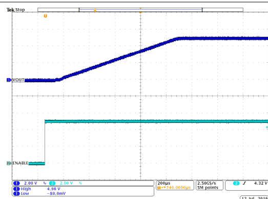
图 10-58. Start-Up Timing
