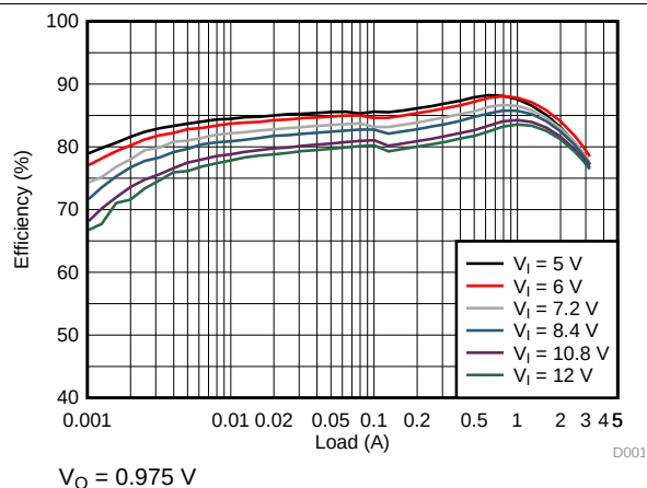
图 5. TPS62134A Efficiency
