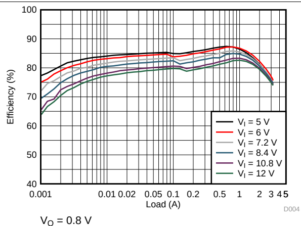
图 8. TPS62134C Efficiency
