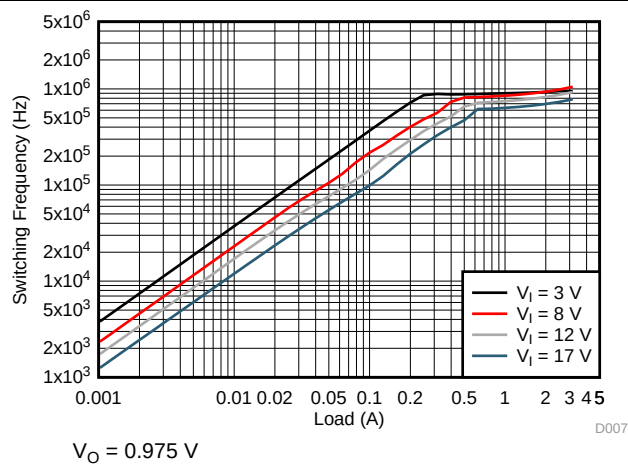
图 11. TPS62134A Switching Frequency
