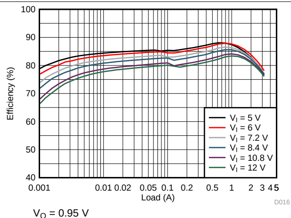
图 6. TPS62134B Efficiency
