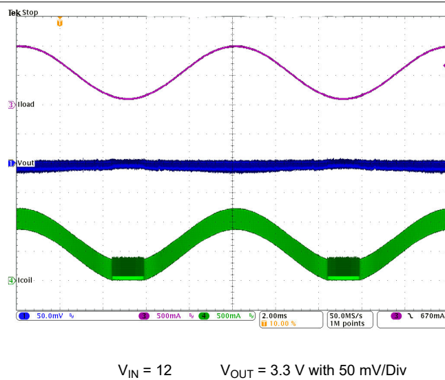
图 9-30. PWM-PSM-Transition
