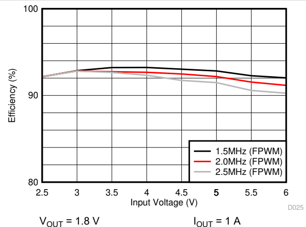
图 9-26. Efficiency with Different Switching Frequency
