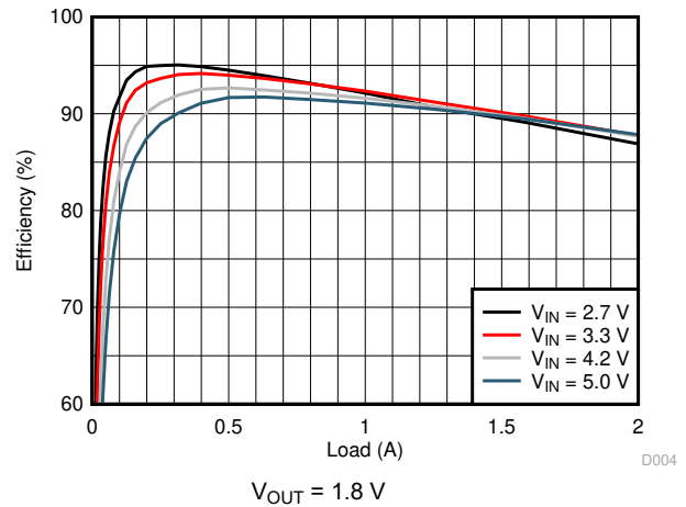
图 9-5. Efficiency, Forced PWM Mode (2.0 MHz)
