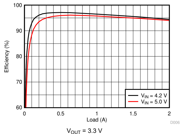
图 9-7. Efficiency, Forced PWM Mode (2.0 MHz)
