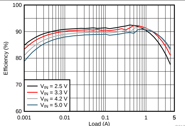
Figure 21. 1.2V Output Application Efficiency
