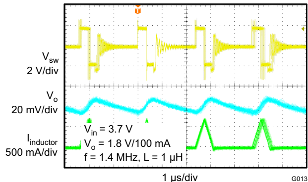
Figure 17. PFM Operation
