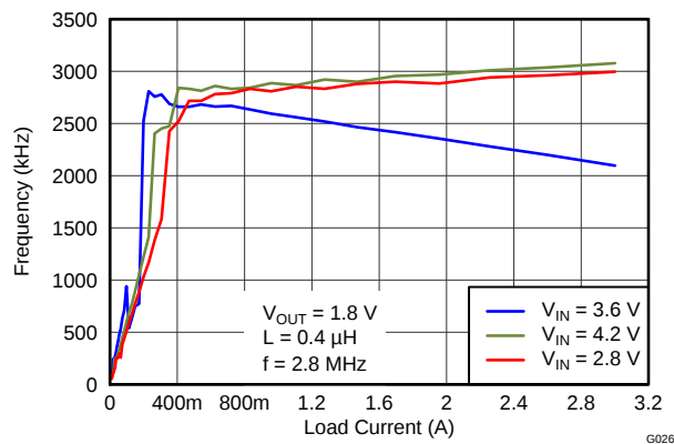
Figure 13. Frequency vs Load Current
