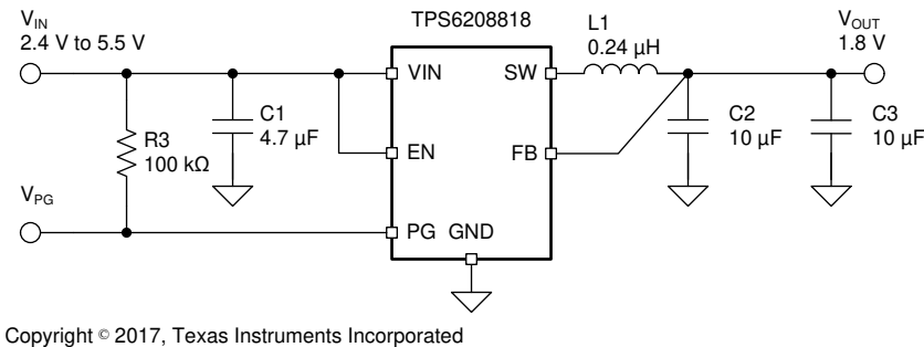
图 8-2. Typical Application of Fixed Output
