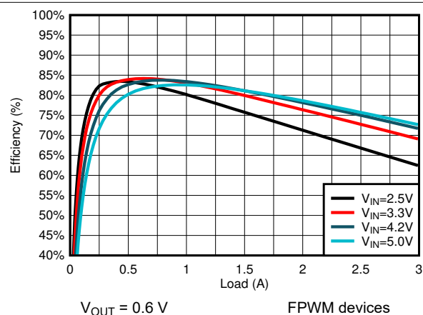
图 8-5. Efficiency
