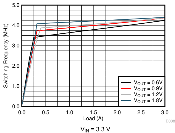
图 8-23. Switching Frequency
