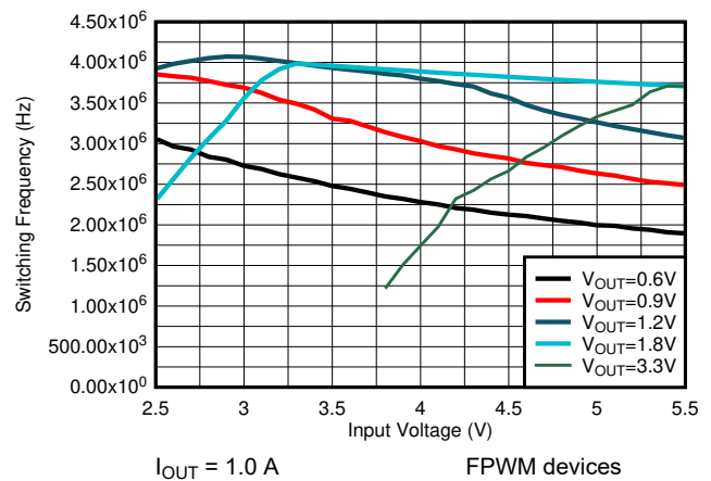
图 8-26. Switching Frequency
