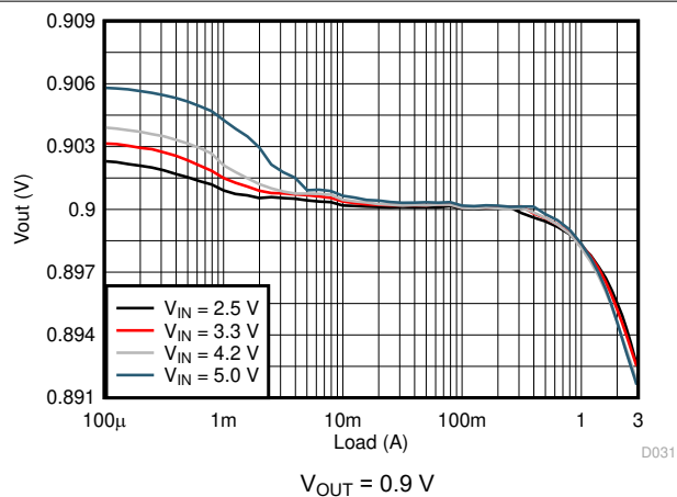
图 8-8. Load Regulation
