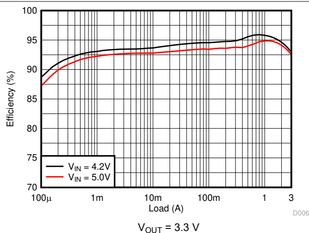
图 8-19. Efficiency
