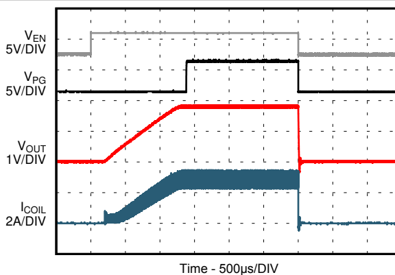
图 8-30. Start-Up With No Load
