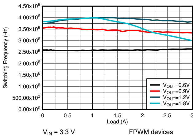
图 8-25. Switching Frequency
