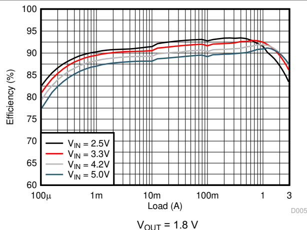
图 8-15. Efficiency
