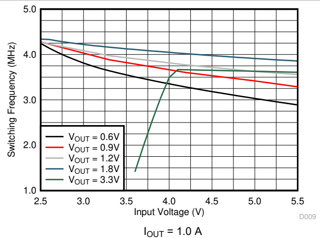
图 8-24. Switching Frequency
