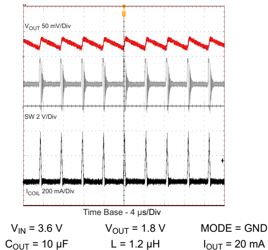
图 10-10. Typical Operation (PFM Mode)
