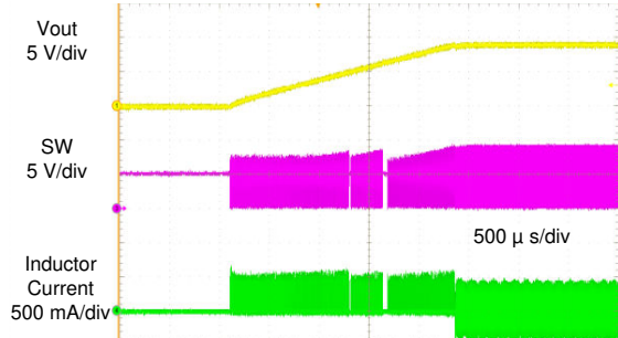
图 9-9. Short Circuit Recovery V_{IN} = 5\text{ V} , V_{OUT} = 9\text{ V} , I_{OUT} = 0\text{ mA} , FPWM
