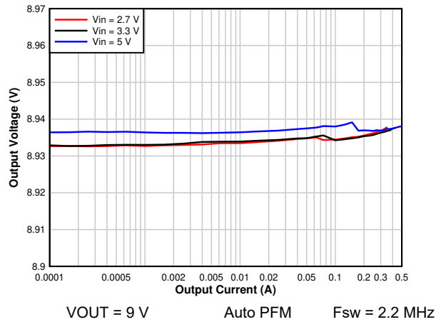
图 7-3. 9 V OUT Regulation vs Output Current
