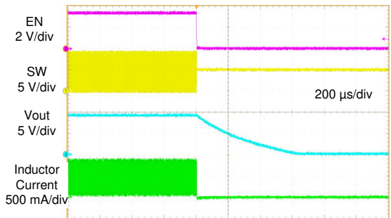
图 9-7. Shutdown from EN Waveforms V_{IN} = 5\text{ V} , V_{OUT} = 9\text{ V} , I_{OUT} = 250\text{ mA} , FPWM
