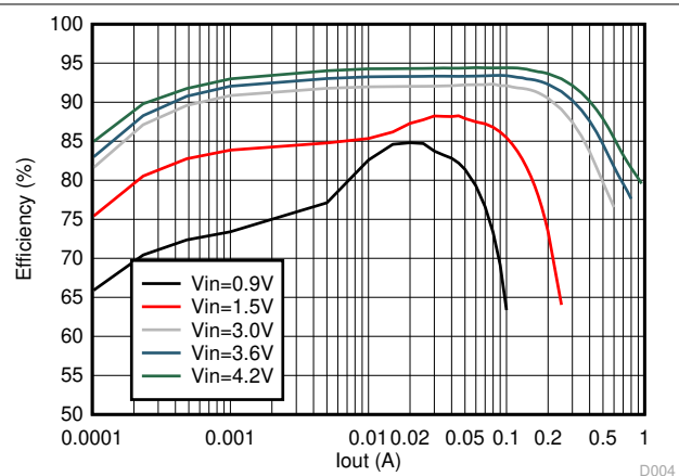
图 6-3. Load Efficiency with Different Inputs
