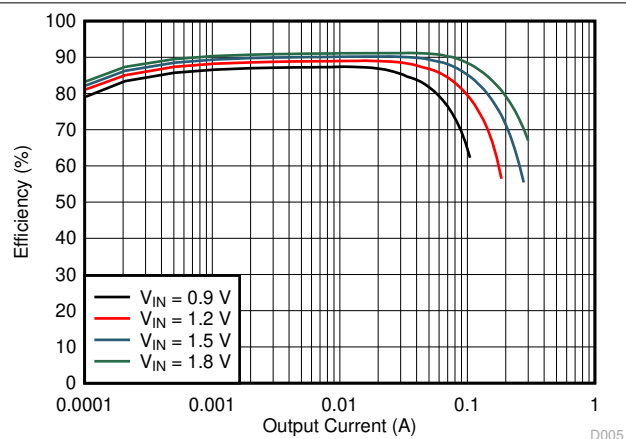
图 6-1. Load Efficiency with Different Inputs
