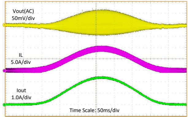
图 9-9. Load Sweep ( I_{OUT} = 0 to 2 \text{ A} )
