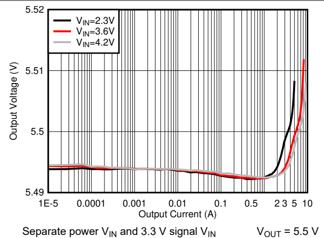
图 7-6. Output Voltage vs Output Current, V_{\text{OUT}} = 5.5\text{ V}
