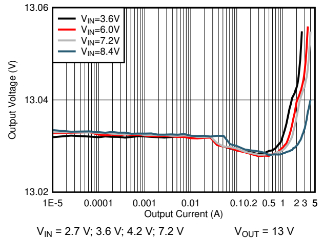
图 7-2. Output Voltage vs Output Current, V_{\text{OUT}} = 13\text{ V}
