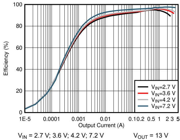
图 7-1. Efficiency vs Output Current V_{\text{OUT}} = 13\text{ V}
