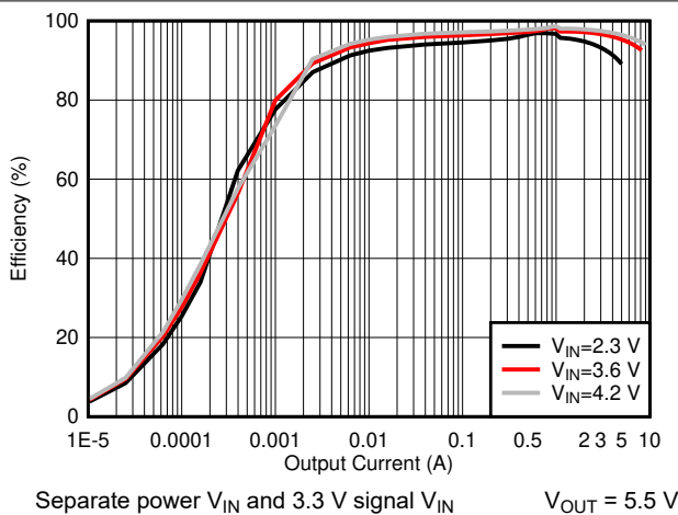
图 7-5. Efficiency vs Output Current, V_{\text{OUT}} = 5.5\text{ V}
