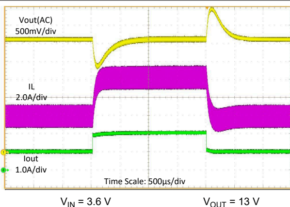
图 9-7. Load Transient ( I_{OUT} = 1\text{ to }2\text{ A} )
