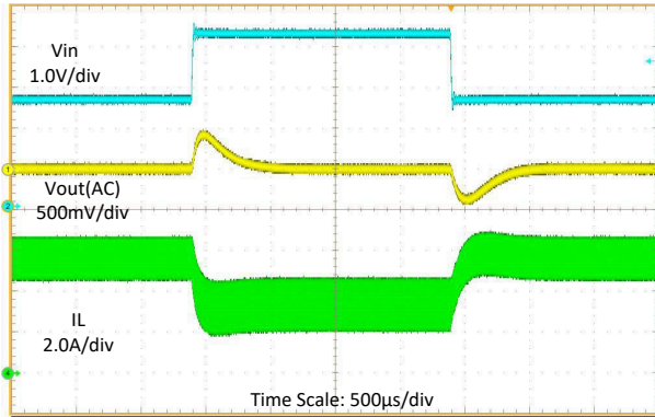
图 9-8. Line Transient ( V_{IN} = 2.7 \text{ V} to 4.2 \text{ V} )
