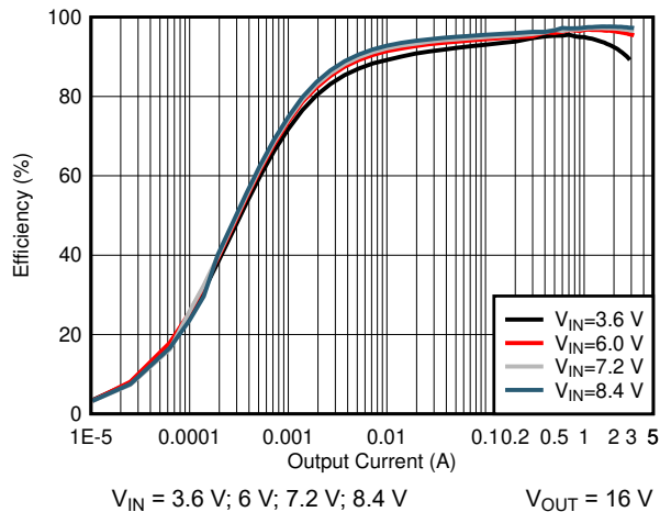
图 7-3. Efficiency vs Output Current, V_{\text{OUT}} = 16\text{ V}
