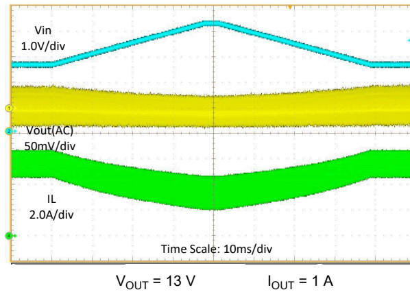
图 9-10. Line Sweep ( V_{IN} = 2.7 \text{ V} to 4.2 \text{ V} )
