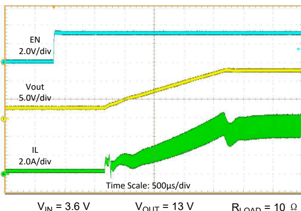
图 9-5. Start-up Waveforms
