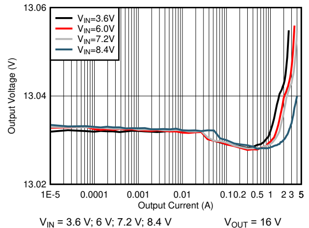
图 7-4. Output Voltage vs Output Current, V_{\text{OUT}} = 16\text{ V}
