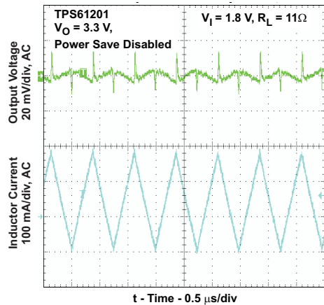
图 16. Output Voltage, Power Save Mode Disabled
