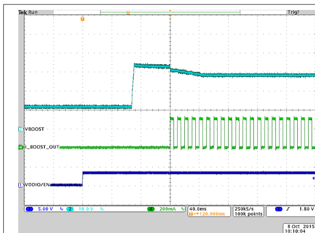
图 8-4. Typical Start-Up
