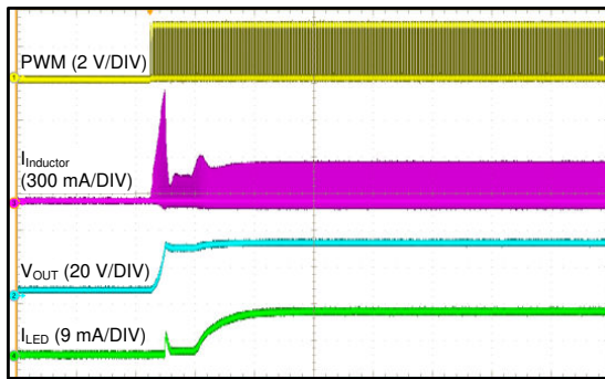
图 7-8. Switching-Dimming Duty = 10%
