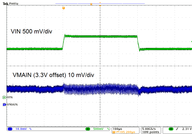
图 9-15. Line Transient Response
