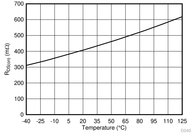
图 7-14. Low Side Switch On Resistance vs Temperature
