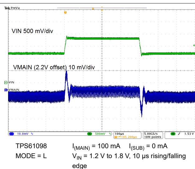
图 9-27. Line Transient Response
