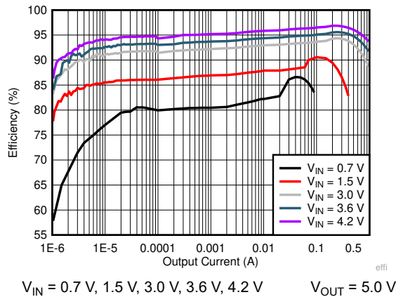
图 6-1. 5.0-V V_{OUT} Efficiency with Different Inputs in Boost Operation
