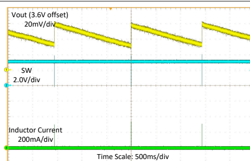
图 8-3. Switching Waveform at Medium Load
