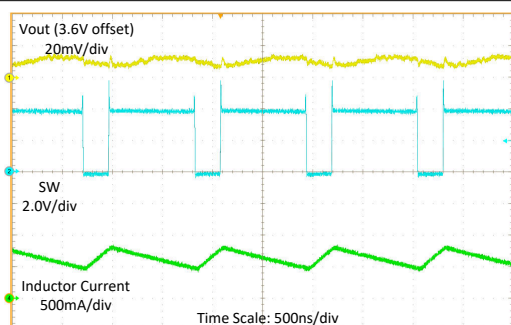
图 8-2. Switching Waveform at Heavy Load
