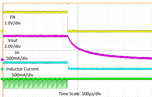
图 8-17. Switching Waveform at Buck Mode with ICHG = 500\text{mA}
