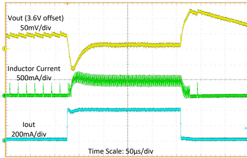
图 8-8. Load Transient at Boost Mode
