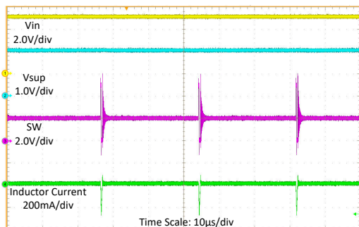
图 8-15. Switching Waveform at Buck Mode with ICHG = 2.5\text{ mA}
