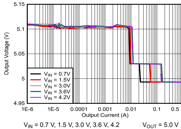
图 6-3. 5.0-V Load Regulation in Boost Operation
