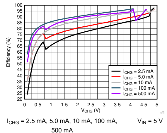
图 6-6. 5-V Input Efficiency with Different Charging current in Buck Operation
