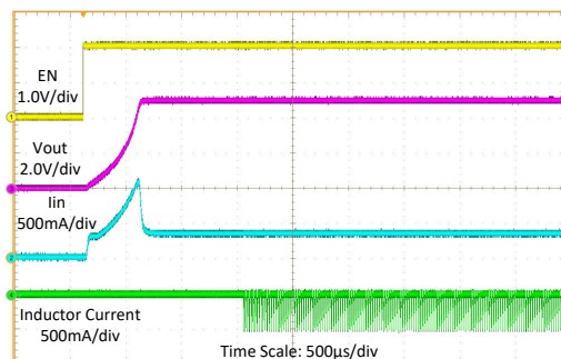
图 8-16. Switching Waveform at Buck Mode with ICHG = 100\text{ mA}
