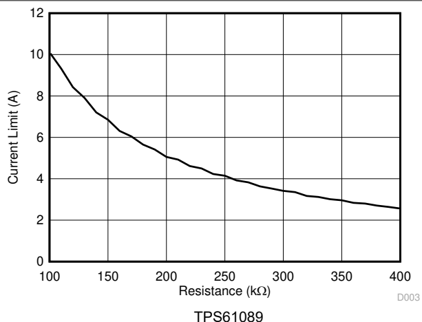
图 7-3. Switching Peak Current Limit Setting
