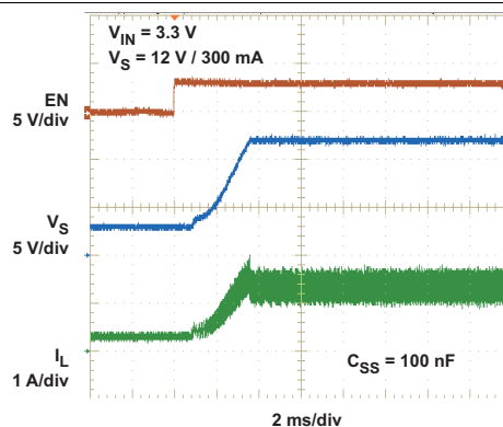
Figure 14. Soft-Start
