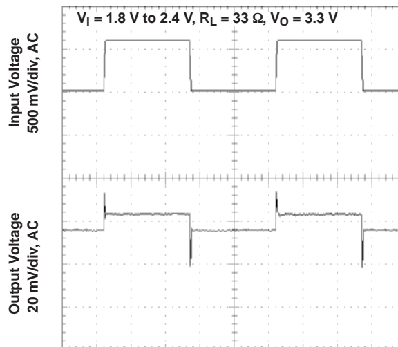
TPS61071 LINE TRANSIENT RESPONSE
