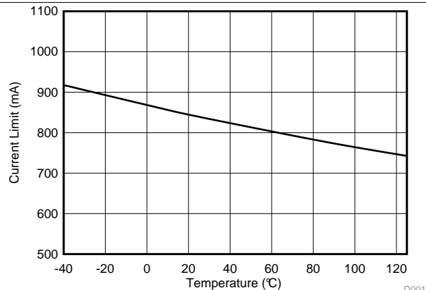
图 8. Current Limit vs Temperature
