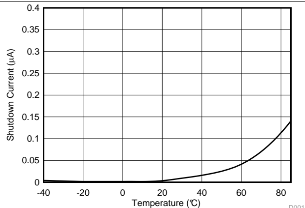
图 7. Shutdown Current vs Temperature
