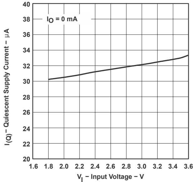
图 7-3. Quiescent Supply Current vs Input Voltage
