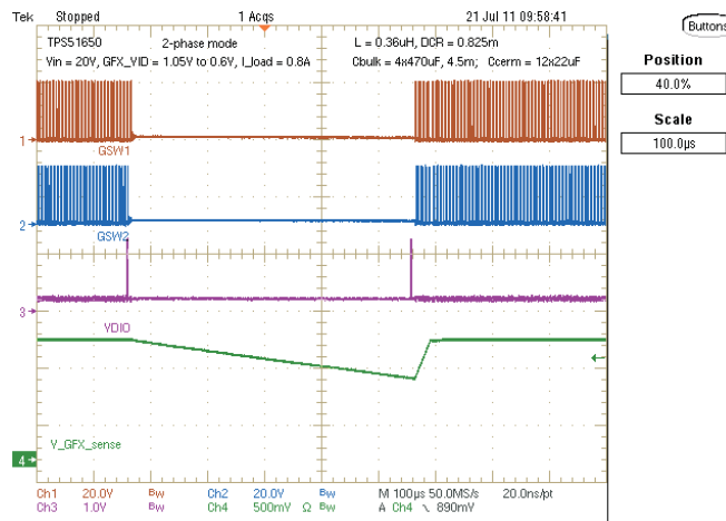
Figure 33. Dynamic VID: V_{IN} = 20\text{ V} , V_{SETVIDSLOW} = 0.6\text{ V} , V_{SETVIDFAST} = 1.05\text{ V}
