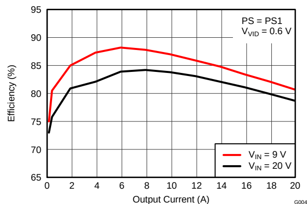
Figure 4. Efficiency vs. Load Current in PS1
