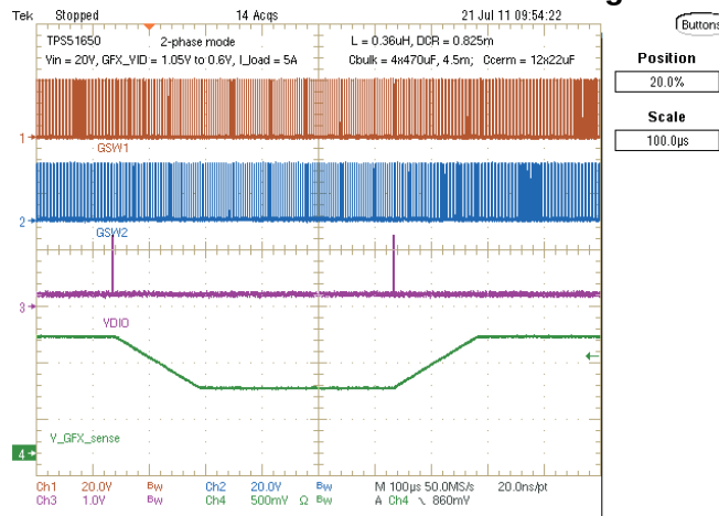
Figure 31. Dynamic VID: V_{IN} = 20\text{ V} , V_{SETVIDSLOW} = 0.6\text{ V} , V_{SETVIDFAST} = 1.05\text{ V}
