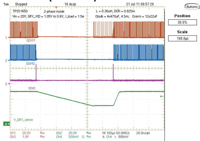
Figure 32. Dynamic VID: V_{IN} = 20\text{ V} , V_{SETVIDSLOW} = 0.6\text{ V} , V_{SETVIDFAST} = 1.05\text{ V}
