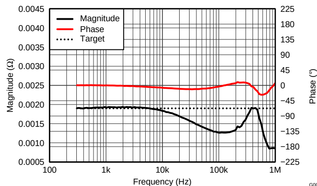
Figure 18. Output Impedance
