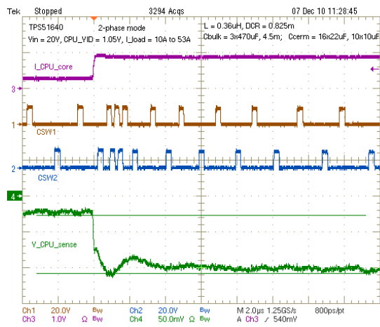
Figure 29. Load Insertion, V_{IN} = 9\text{ V} , Load Step = 43 A, OSR/USR Setting 39 kΩ (Reduced Output Capacitance)
