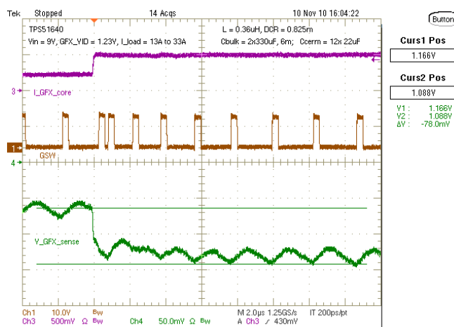
Figure 47. Load Insertion, V_{IN} = 9V , Load Step = 20 A
