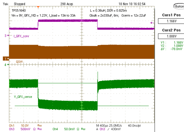
Figure 45. Load Transient, V_{IN} = 9V , Load Step = 20 A
