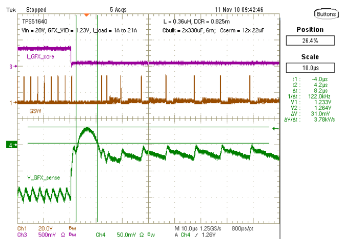
Figure 48. Load Release, V_{IN} = 20V , Load Step = 20 A
