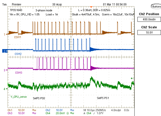
Figure 16. PS Change PS0 to PS1 Toggle
