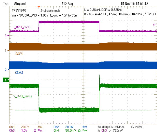
Figure 25. Load Transient, V_{IN} = 9\text{ V} , Load Step = 43 A
