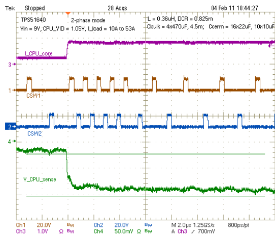
Figure 27. Load Insertion, V_{IN} = 9\text{ V} , Load Step = 43 A, OSR/USR Setting 150 kΩ
