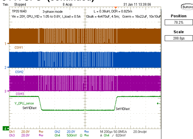
Figure 14. Dynamic VID: SetVID-Fast/SetVID-Fast
