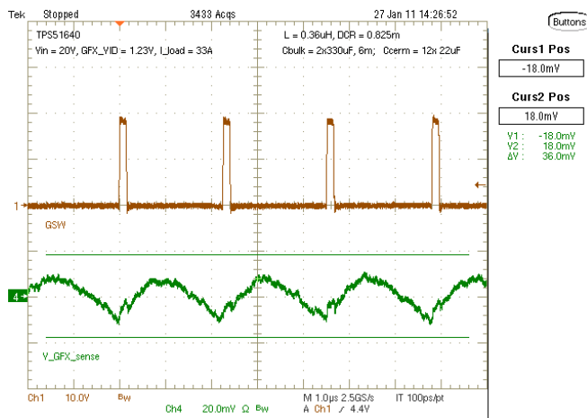
Figure 42. Switching Ripple in PS0
