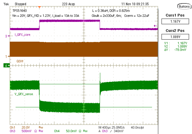
Figure 46. Load Transient, V_{IN} = 20V , Load Step = 20 A
