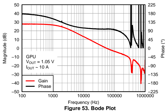
Figure 53. Bode Plot
