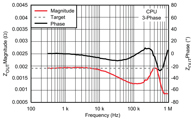
Figure 18. Output Impedance
