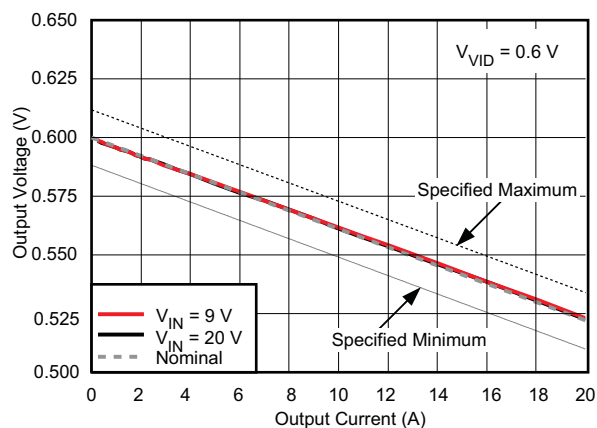
Figure 38. Output Voltage Vs. Load Current in PS1
