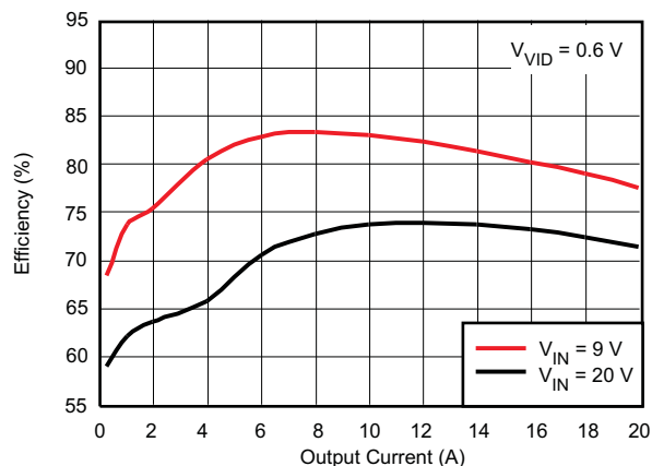
Figure 40. Efficiency Vs. Load Current in PS1
