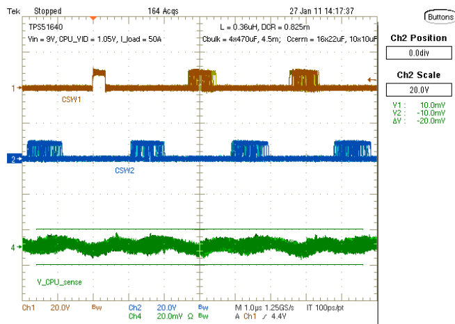
Figure 21. Switching Ripple in PS0 (Persistence), V_{IN} = 9\text{ V}
