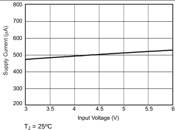
图 15. Shutdown Supply Current versus Input Voltage
