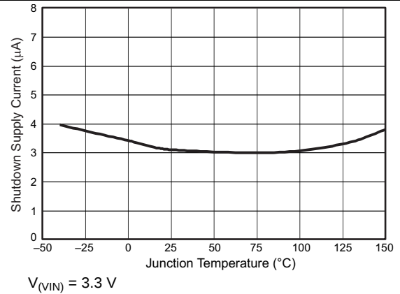
图 14. Shutdown Supply Current versus Temperature
