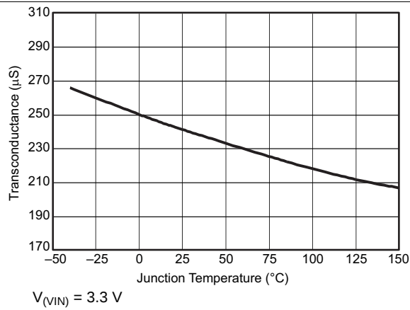
图 7. Transconductance versus Temperature
