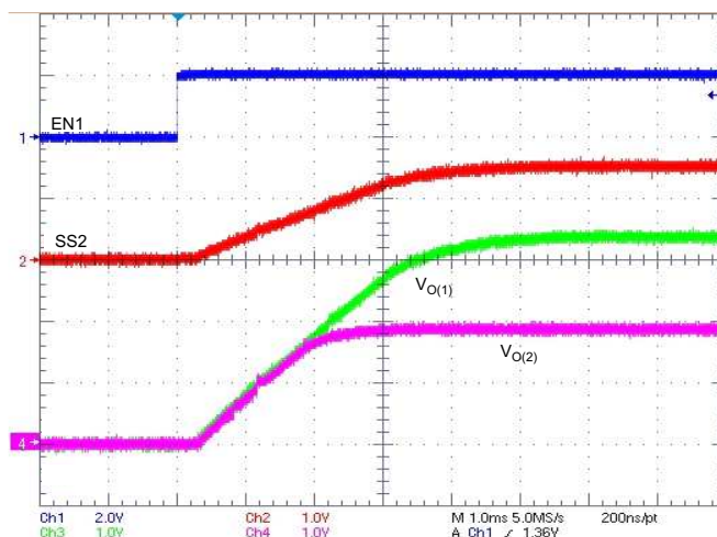
图 28. Ratiometric Start-Up Using Coupled SS/TR Pins
