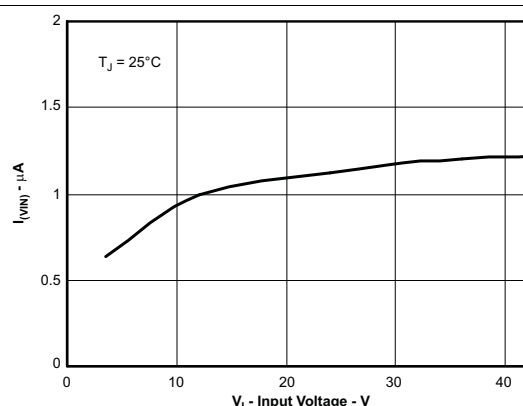
Figure 16. Shutdown Supply Current vs Input Voltage ( V_{IN} )
