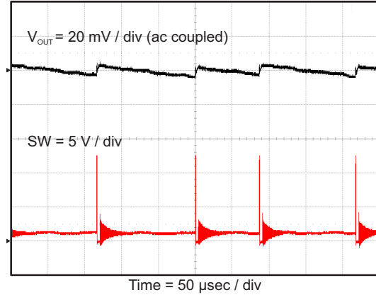
图 32. Output Voltage Ripple, I_{OUT} = 10\text{ mA}
