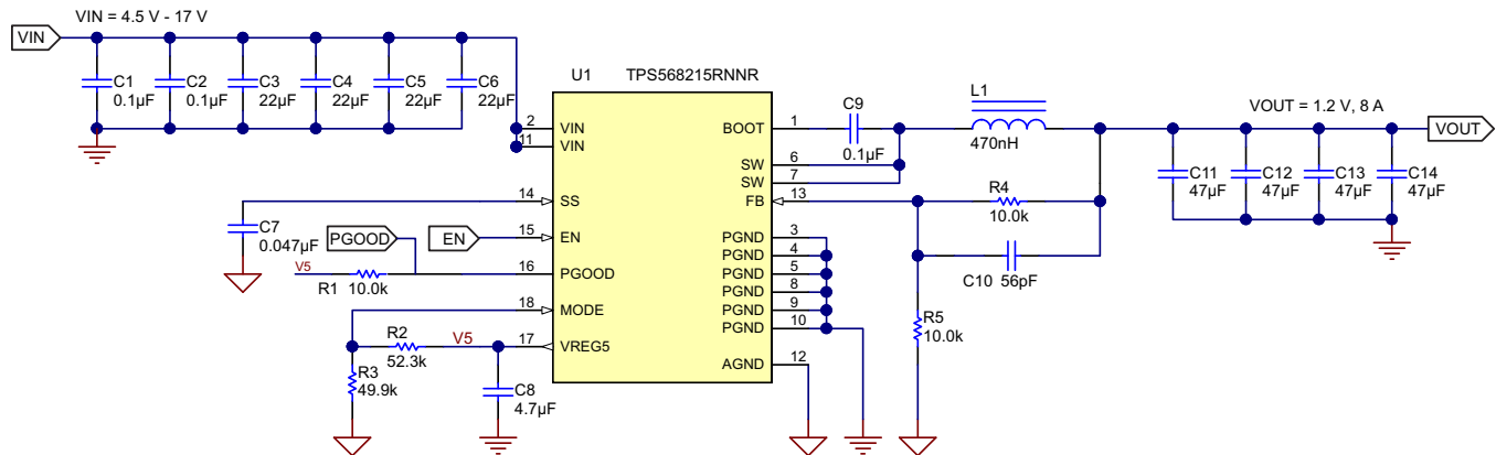
图 22. Application Schematic
