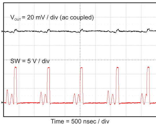
图 8-12. Output Voltage Ripple, I_{OUT} = 700 mA
