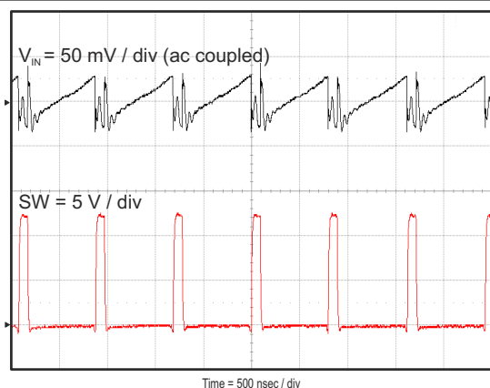
图 8-10. Input Voltage Ripple, I_{OUT} = 8 A
