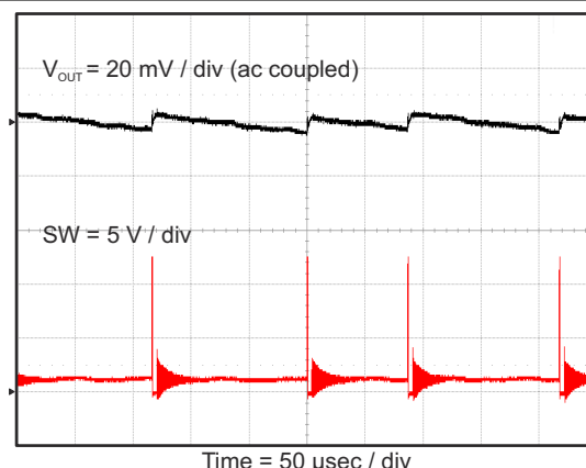
图 8-11. Output Voltage Ripple, I_{OUT} = 10 mA
