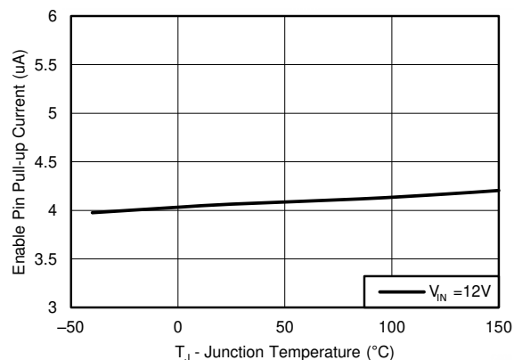
图 6-8. Enable Pull-Up Current, V_{EN} = 1.3V
