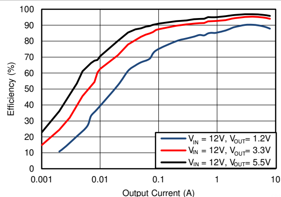
图 6-12. Efficiency, Mode = DCM, F_{SW} = 400kHz
