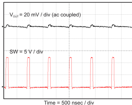
图 8-13. Output Voltage Ripple, I_{OUT} = 8 A
