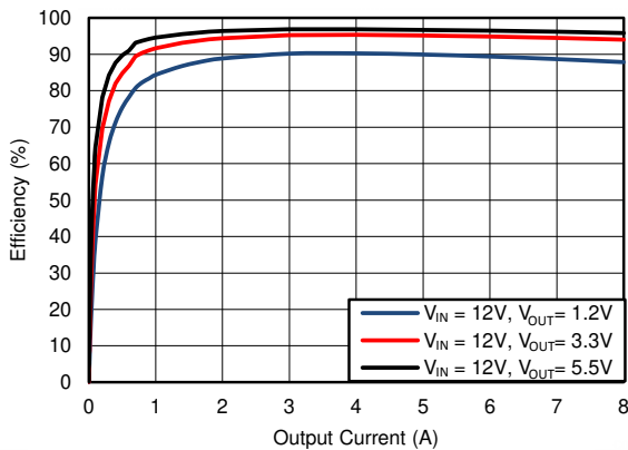
图 6-13. Efficiency, Mode = FFCM, F_{SW} = 400\text{kHz}
