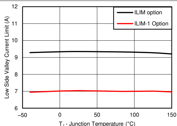
图 6-10. Valley Current Limit vs Temperature
