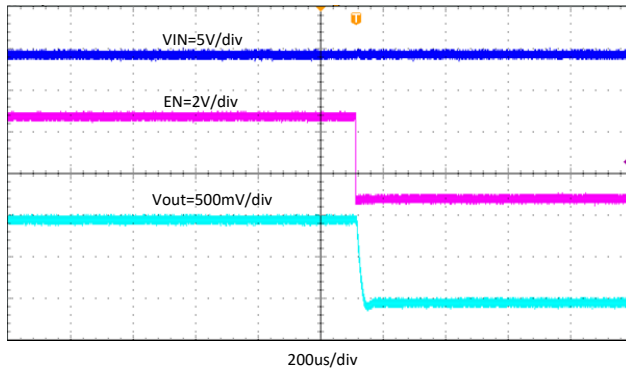
图 7-16. Shutdown Through EN, I_{OUT} = 3\text{ A}
