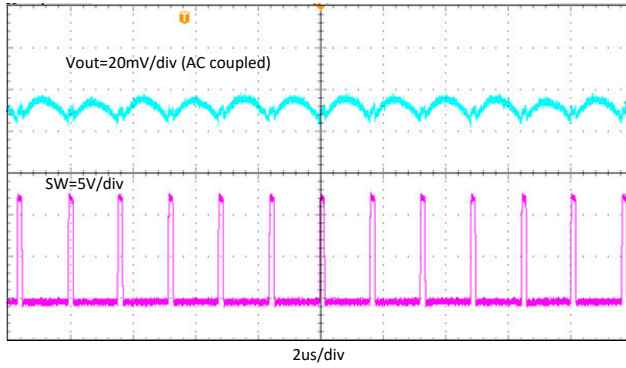
图 7-14. Output Voltage Ripple, I_{OUT} = 6\text{ A}
