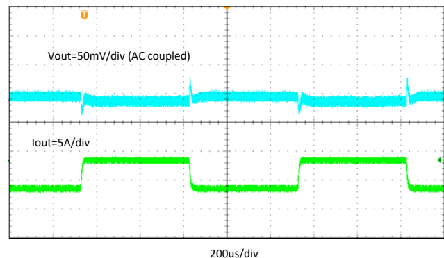
0.6 A to 5.4 A Slew Rate = 2.5\text{ A}/\mu\text{s} 图 7-19. TPS566231 Transient Response
