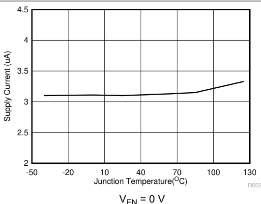
图 5-3. Shutdown Current vs Temperature
