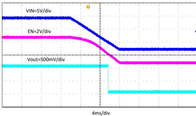
图 7-18. Start-Up with V_{IN} Falling, I_{OUT} = 3\text{ A}
