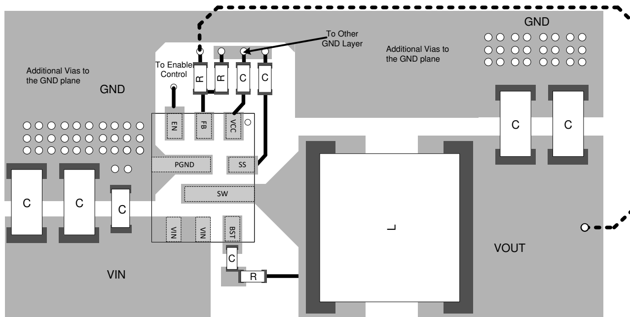
图 7-26. Top-Layer Layout
