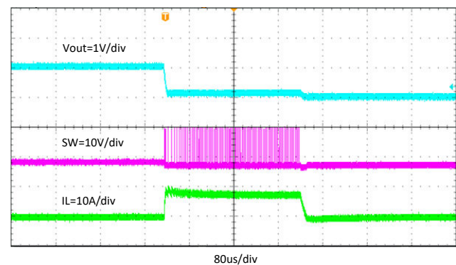
图 7-23. TPS566231 Normal Operation to Output Hard Short
